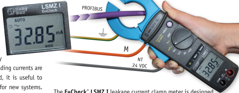
EmCheck® LSMZ I
