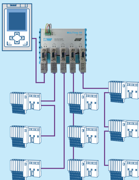
Fig. 20: Star network application example
