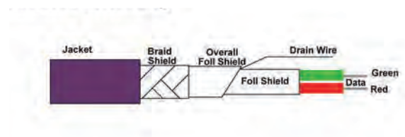
Engineering drawing
