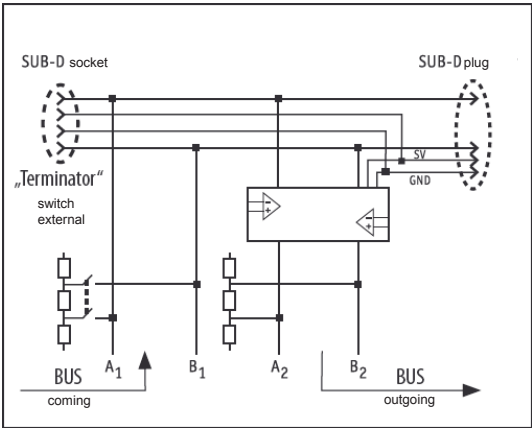
Interface diagram
