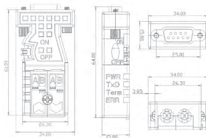
Engineering drawing
