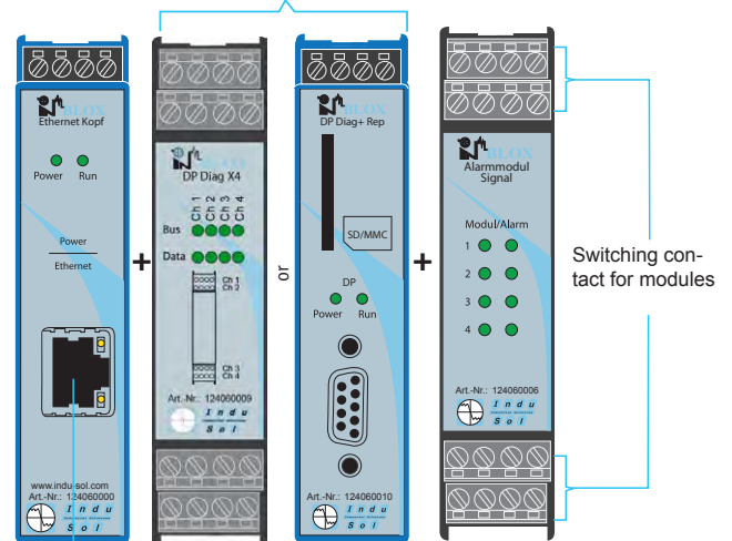
Sample configuration
