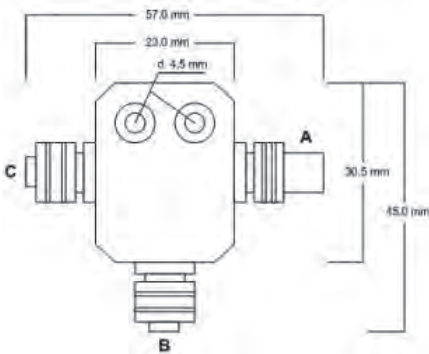
Engineering drawing
