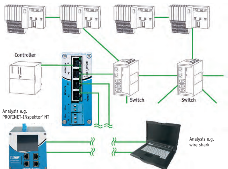
Example of topology - temporary telegram analysis
