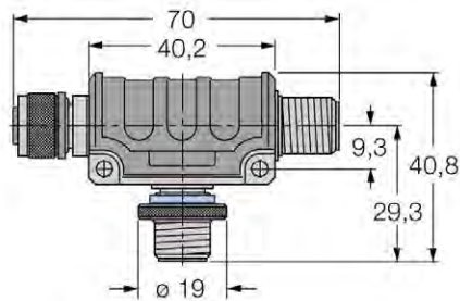
Engineering drawing
