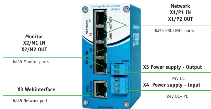
Device ports
