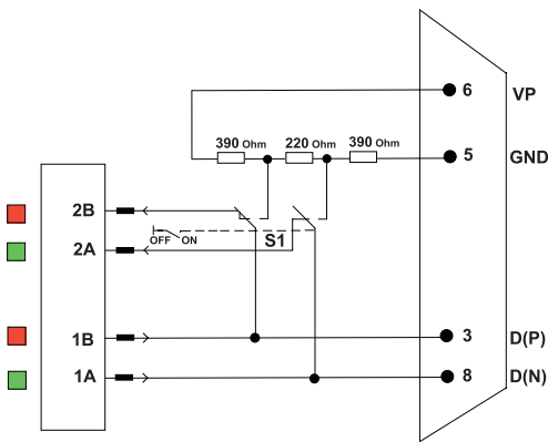
Functional diagram
