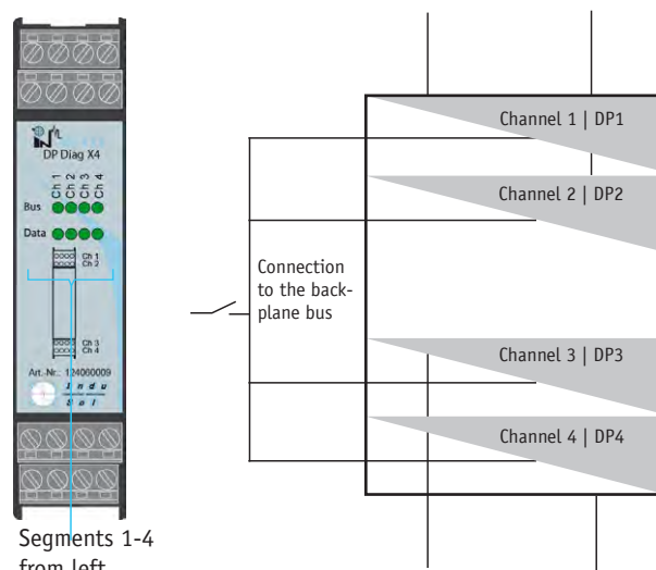
Sample configuration
