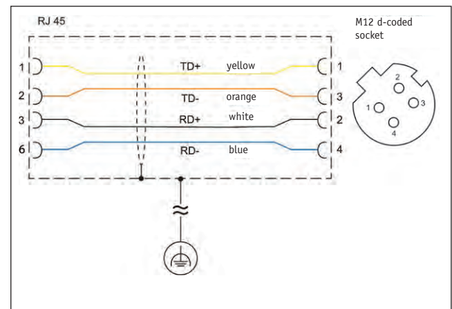
Functional diagram
