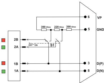
Functional diagram
