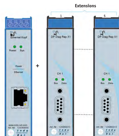
Sample configuration
