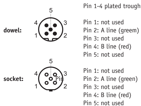
Pin assignment
