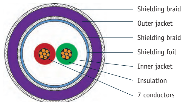
Cross section PROFIBUS cable +FE flexible
