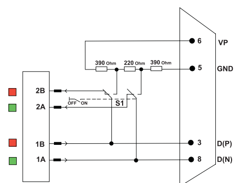
Functional diagram
