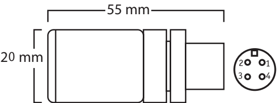
Engineering drawing ASi plug 2
