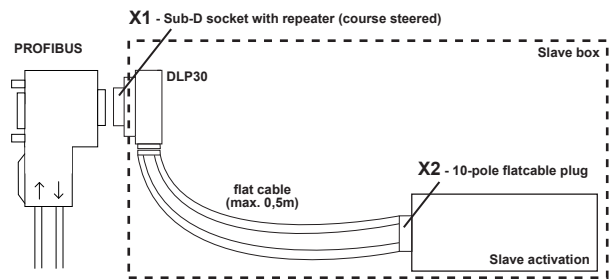
Engineering drawing
