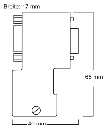
Engineering drawing
