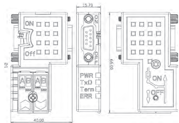
Engineering drawing
