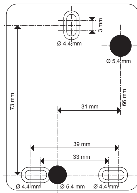
Engineering drawing
