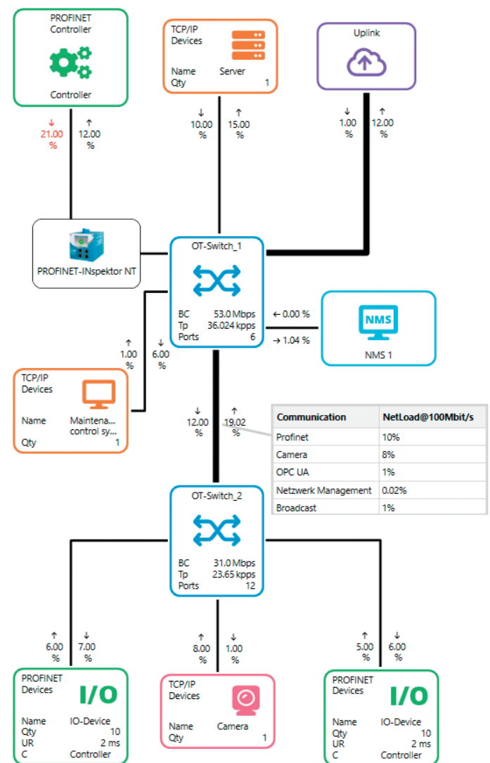
Topology view
