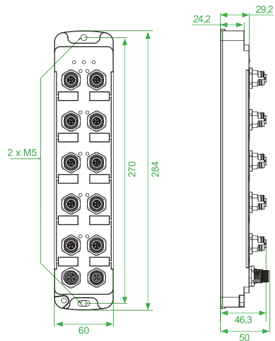
Dimensions (mm)
