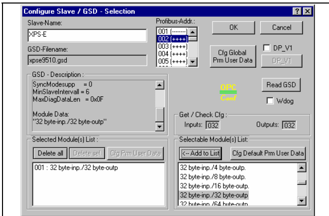
Figure 40: Slave-Configuration Dialogue
