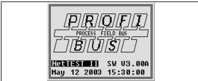
Figure 2: Screen 'Start-up'
