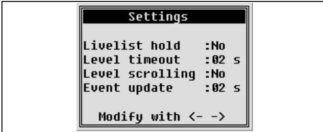
Figure 74: Screen 'Settings'
