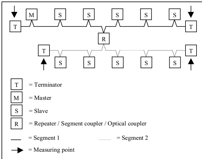
Figure 1: Connection NetTEST II in the cable thread
